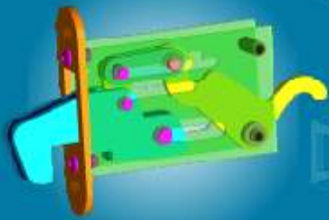
Gladiator locking mechanism
